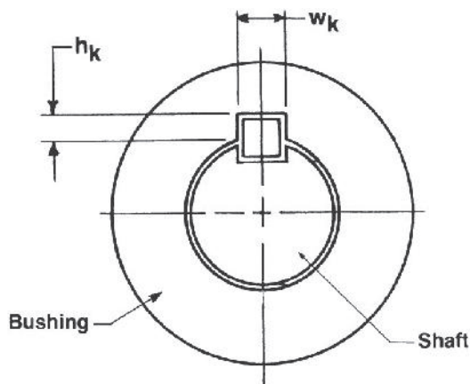
Standard Shaft and Bushing Keyseat Dimensions
